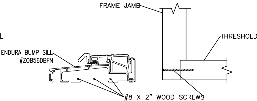
11 THRESHOLD TO FRAME DETAIL
