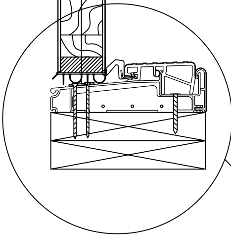
A STILE DOOR SECTION WOOD SUBSTRATE INSTALLATION
