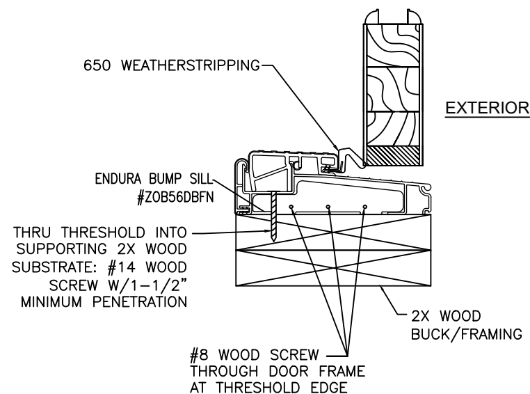
6 THRESHOLD SECTION AT SILL
