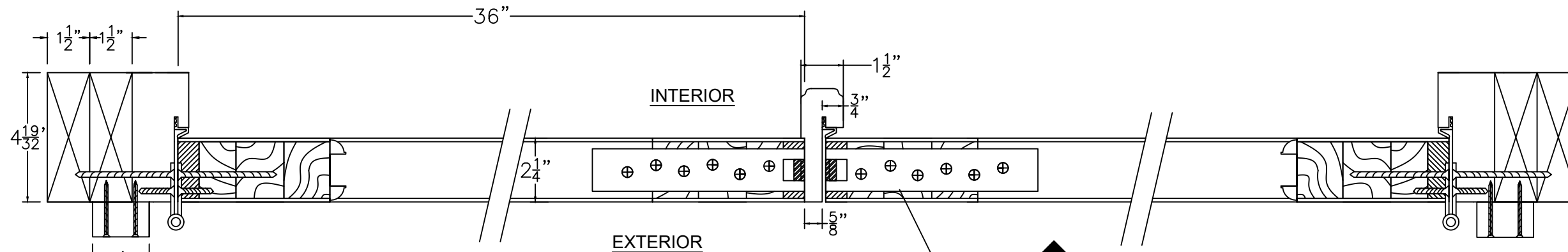
(A) TOP RAIL SECTION WOOD SUBSTRATE INSTALLATION
