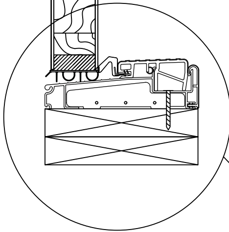
B GLAZED DOOR SECTION WOOD SUBSTRATE INSTALLATION
