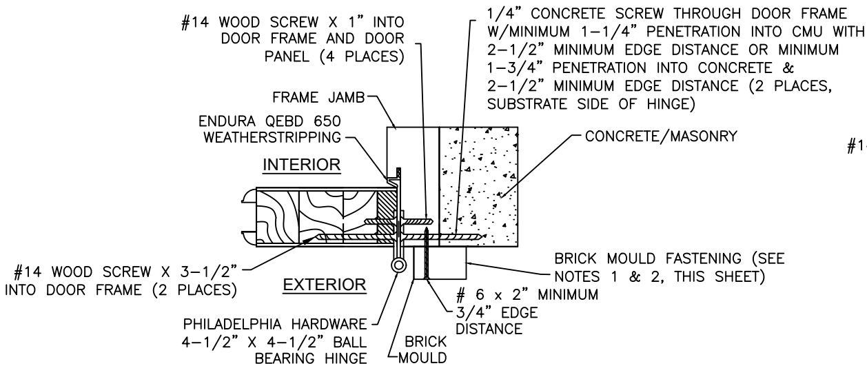
8 JAMB ANCHORAGE @ HINGE
