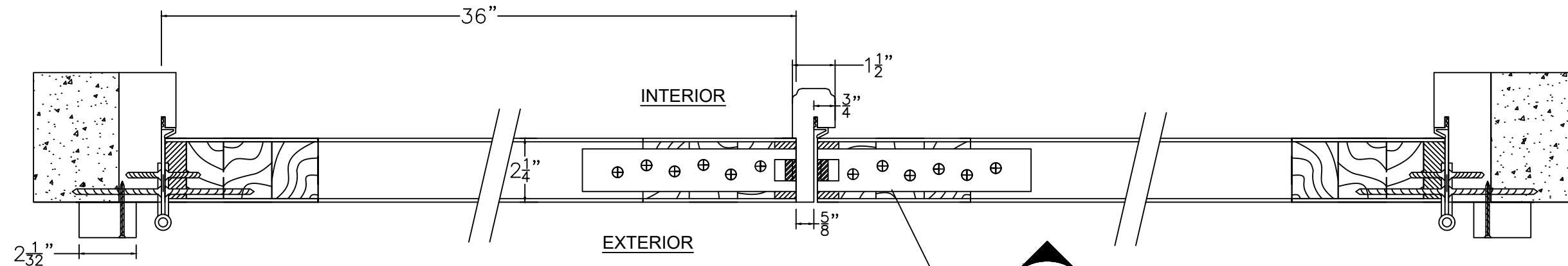
A TOP RAIL SECTION CONCRETE/MASONRY SUBSTRATE INSTALLATION
